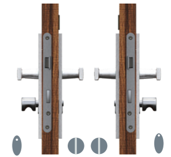
Knob-Coin type cylinder Coin-Knob type cylinder
